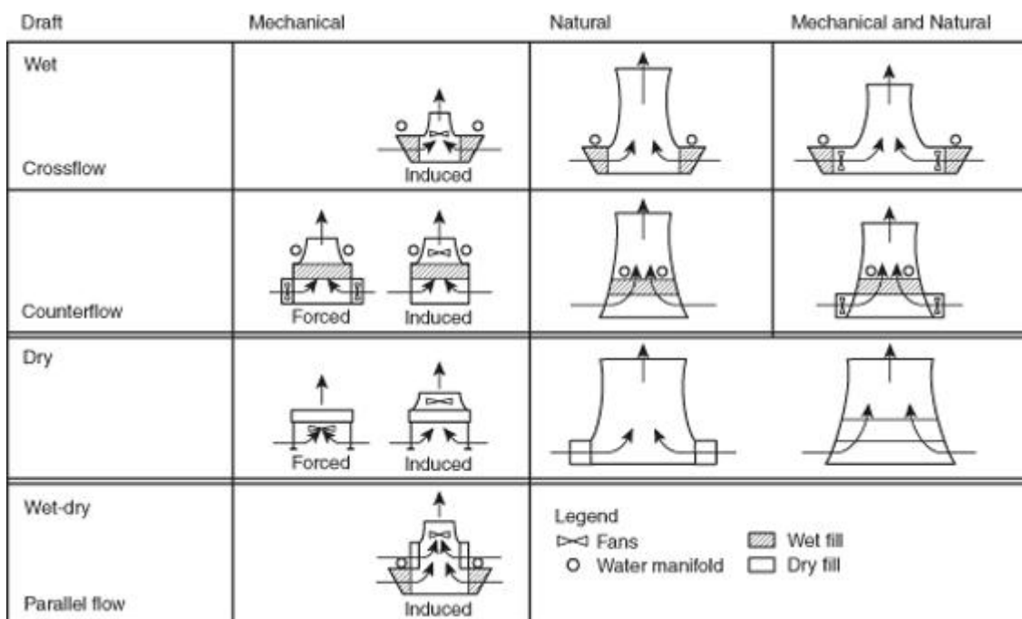
FIGURE B.1(a) Summary of Typical Water-Cooling Towers. (Courtesy of FM Global)
