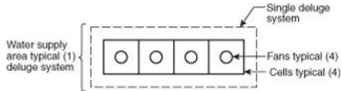
FIGURE A.5.6.1.1 Single Deluge System.
