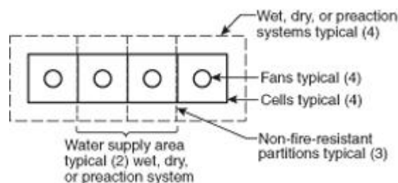
FIGURE A.5.6.2.2 Multiple Wet, Dry, or Preaction Systems with No Fire-Resistant Partitions.
