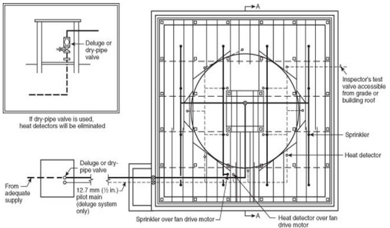
FIGURE A.5.2.4.1(c) Plan View, Typical Deluge or Dry-Pipe Fire Protection Arrangement for Counterflow Towers.
