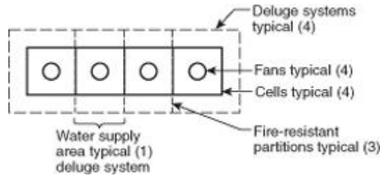
FIGURE A.5.6.1.3 Multiple Deluge Systems.
