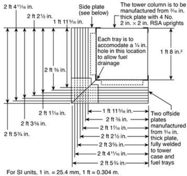
FIGURE D.1(e) Plan View of the Fire Tower (Omitting the Upper Flange for Clarity).
