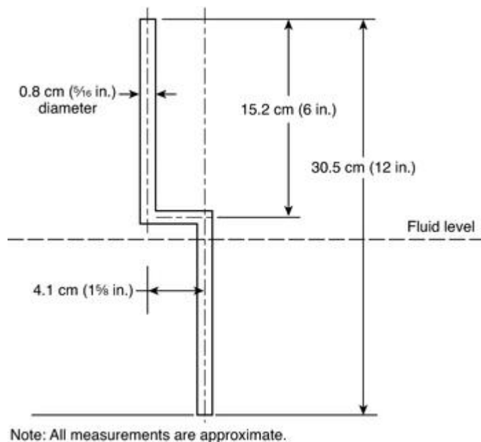
FIGURE 5.2.2.2 Stirrer Shaft for Miscibility Test.
