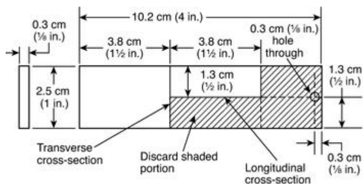
FIGURE 5.3 Intergranular Corrosion Test.
