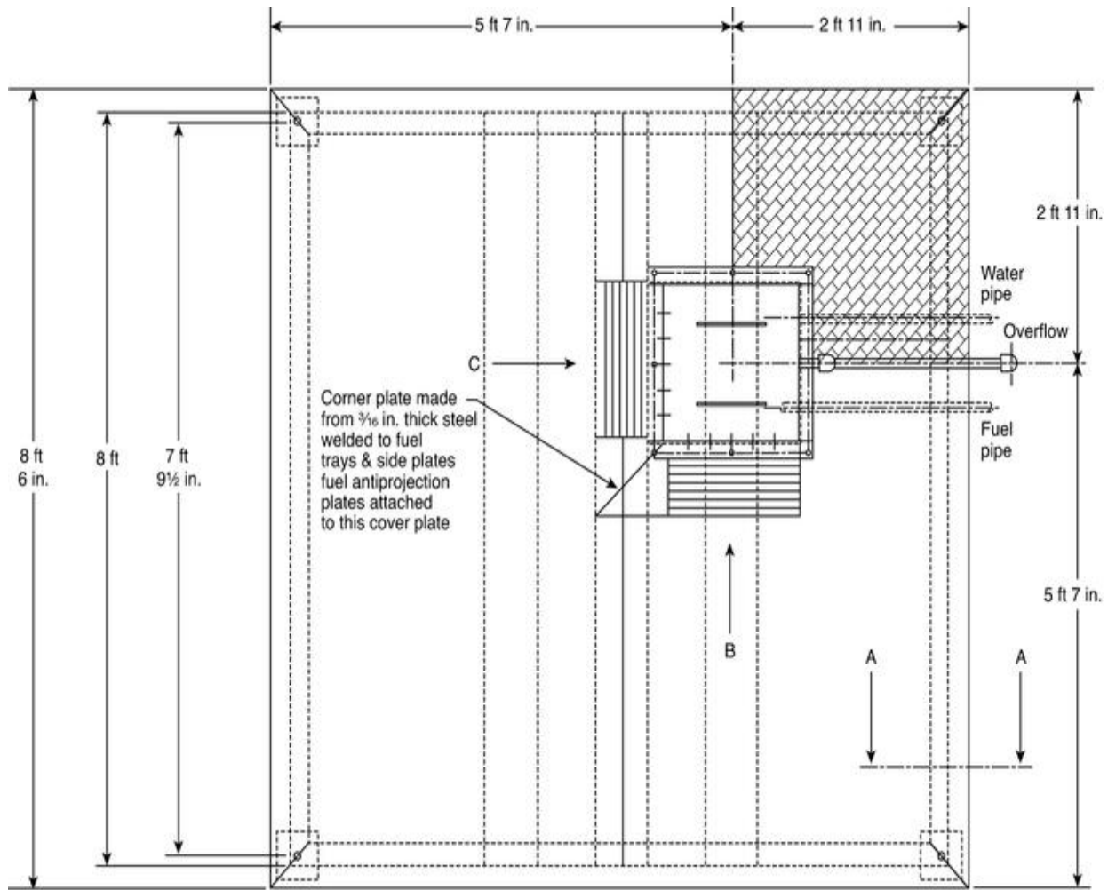
FIGURE D.1(c) Plan View of the Fire Tower and Water Trough.
