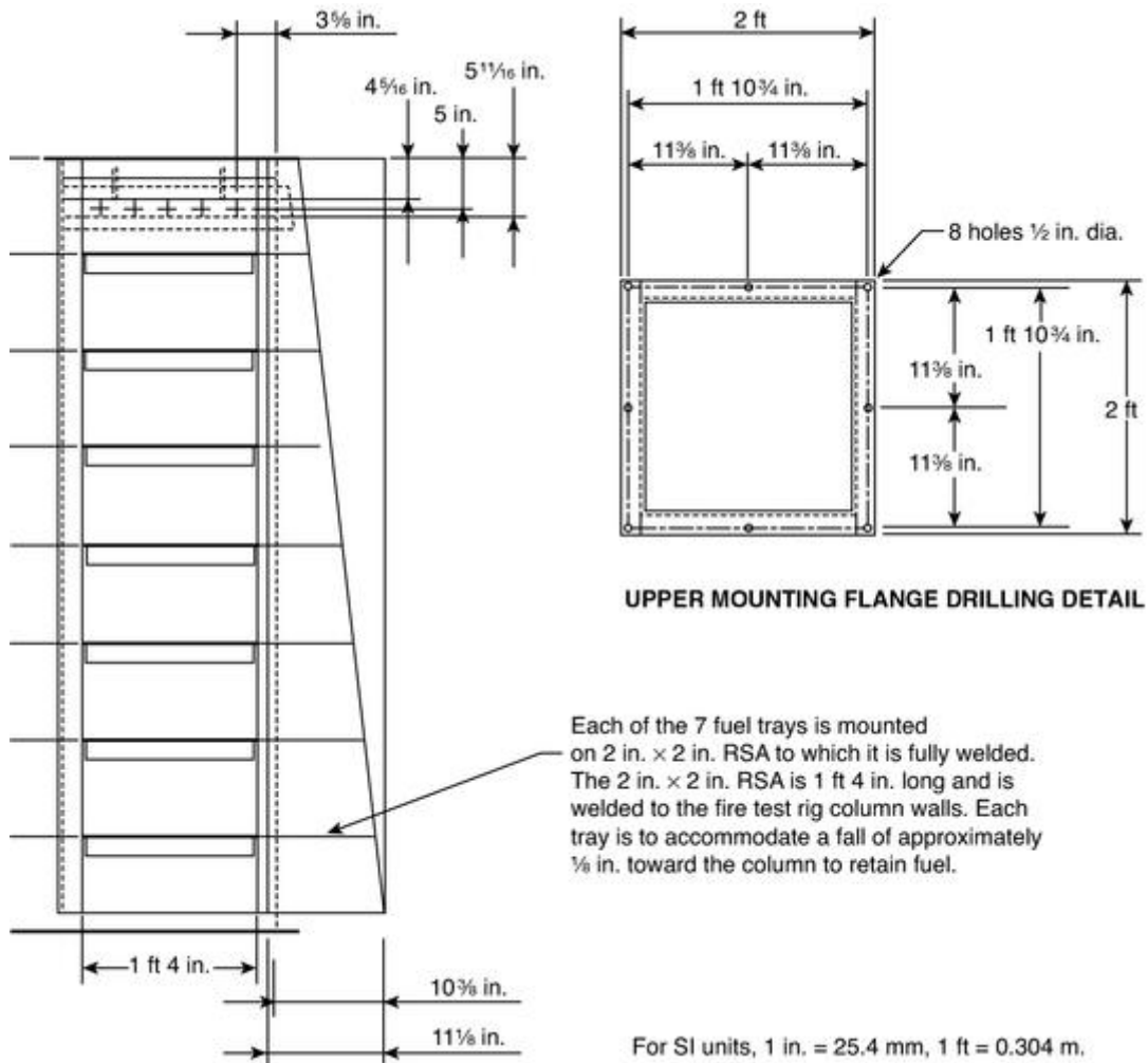
FIGURE D.1(d) Side Elevation of the Fire Tower (Omitting the Water Trough for Clarity).
