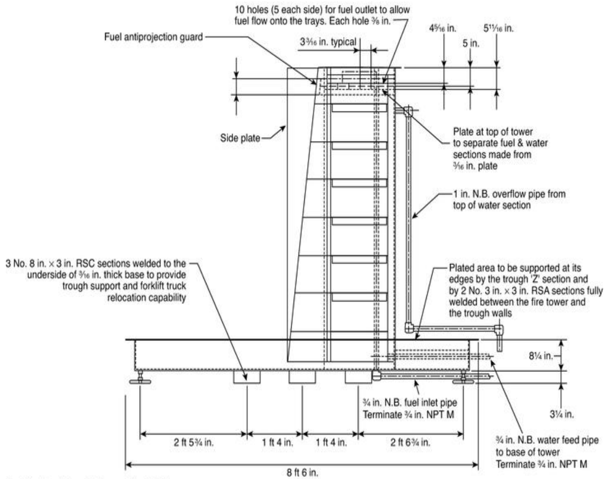
FIGURE D.1(b) FAA — Running Fuel Fire Cascade, 2.4 m × 2.4 m (8 ft × 8 ft) Basin — Tower 0.6 m × 0.6 m (2 ft × 2 ft) Side Elevation on the Fire Tower and Water Trough.
